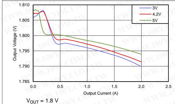
Figure 22. Regulation, AUTO Mode
