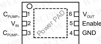
TQFN (TOP VIEW)
