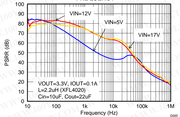
Figure 27. Power Supply Rejection Ratio, f_{SW}=2.5\text{MHz}
