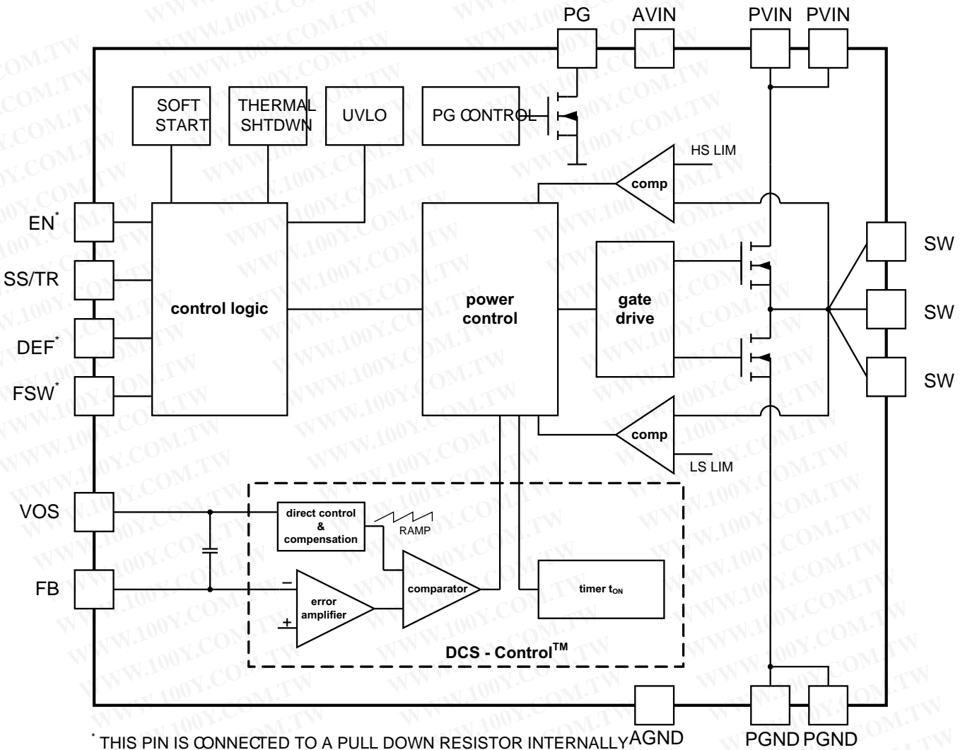
Figure 2. TLV62130
