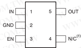
DDC PACKAGE TSOT23-5 (TOP VIEW)
