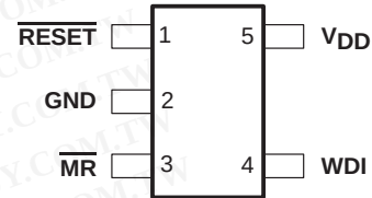
TPS3824 . . . DBV PACKAGE
