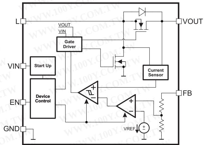
Functional Block Diagram (Fixed Output Voltage Version)
