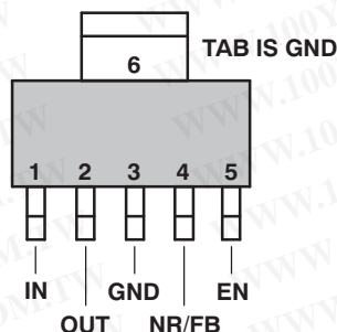
DCQ PACKAGE SOT223 (TOP VIEW)
