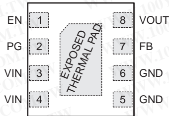
Pin Functions
