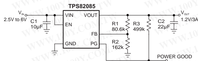
Figure 4. 1.2-V Output Application
