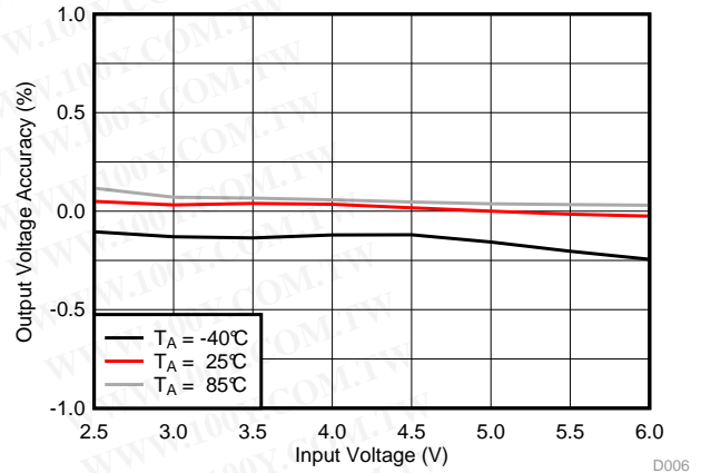
Figure 12. Line Regulation
