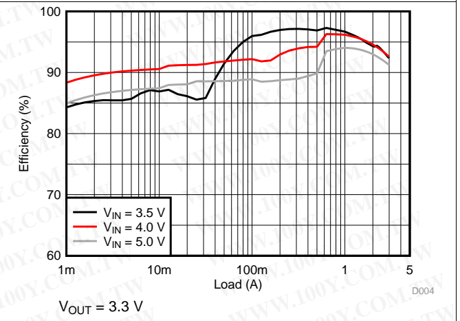
Figure 8. Efficiency
