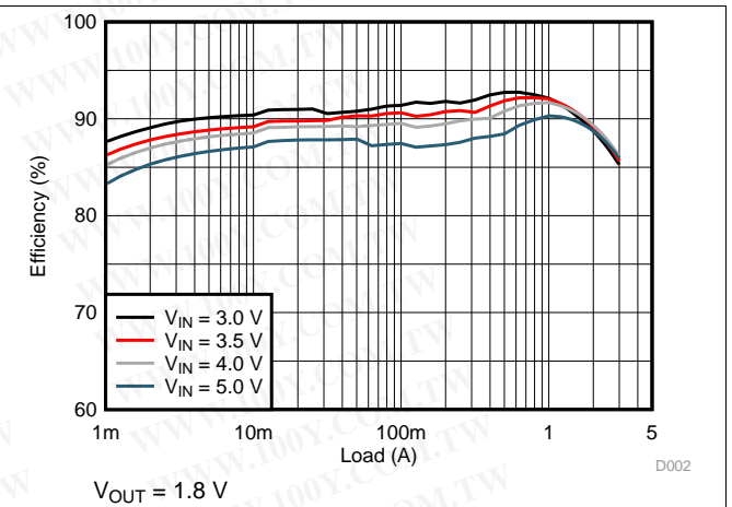
Figure 6. Efficiency
