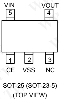
[XC6211 Series]
