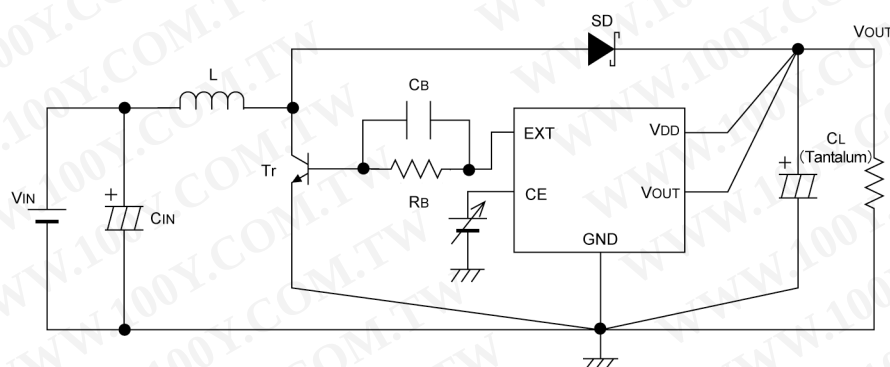
Circuit 8. XC6367B, XC6368B (NPN Transistor)
