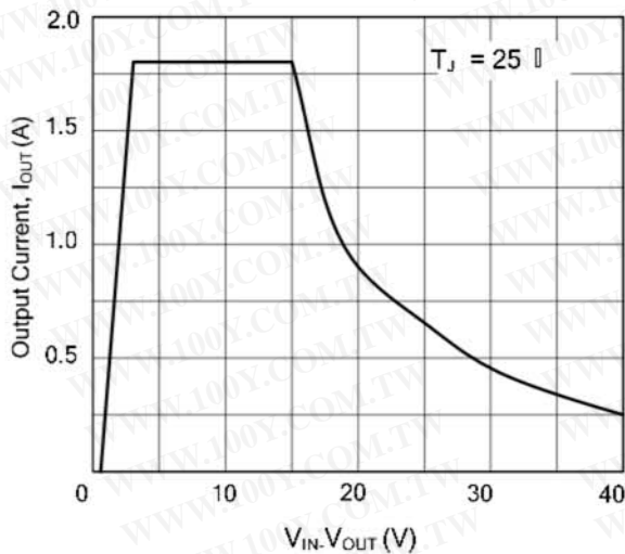
Current Limit
