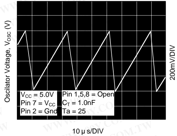
Figure 2. Timing Capacitor Waveform
