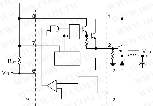
2a. External NPN Switch
