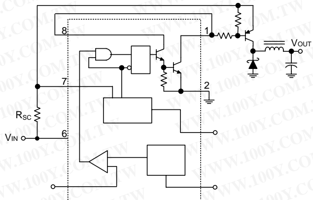
2b. External PNP Saturated Switch
