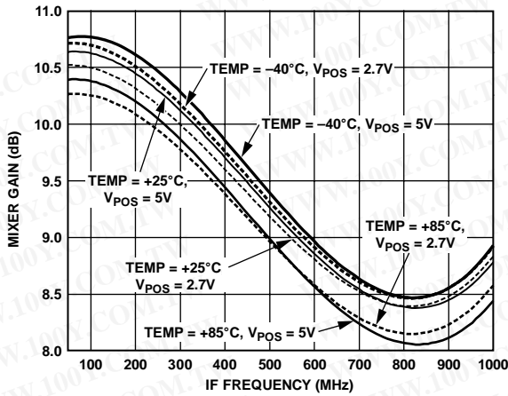
Figure 30. Mixer Gain vs. F_{IF} , V_{POS} = 2.7\text{ V}, 5\text{ V} , F_{BB} = 1\text{ MHz} , Temperature = -40°C, +25°C, +85°C
