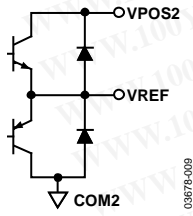
Figure 9. Circuit G
