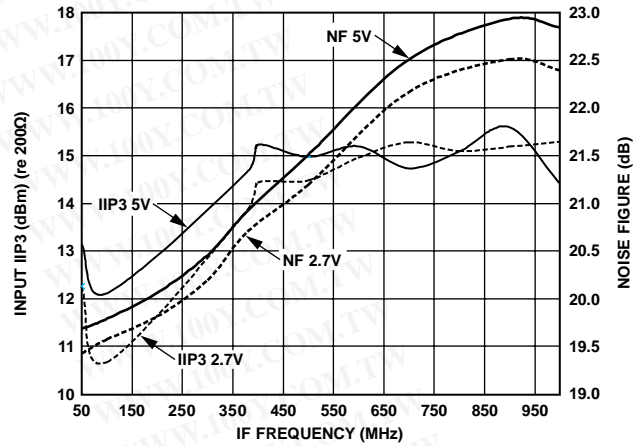
Figure 32. IIP3 and Noise Figure vs. F_{IF} , V_{POS} = 2.7\text{ V}, 5\text{ V} , Temperature = 25°C
