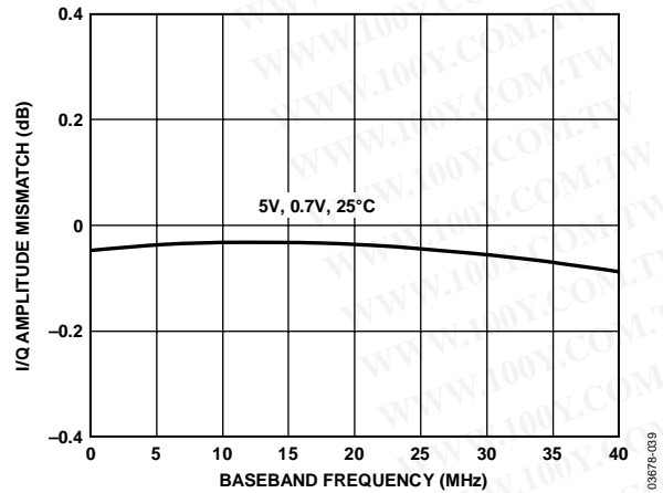
Figure 39. I/Q Amplitude Imbalance vs. F_{BB} , Temperature = 25^{\circ}C , V_{POS} = 5 V
