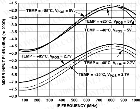
Figure 31. Input 1 dB Compression Point vs. F_{IF} , F_{BB} = 1\text{ MHz} , V_{POS} = 2.7\text{ V}, 5\text{ V} , Temperature = -40°C, +25°C, +85°C
