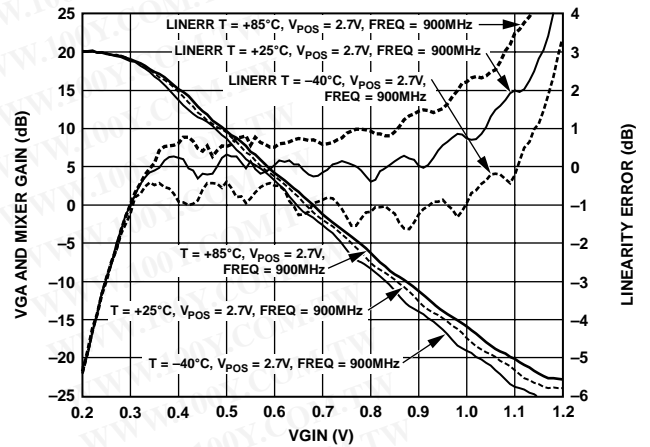
Figure 15. Mixer Gain and Linearity Error vs. VGIN, V_{POS} = 2.7V , F_{IF} = 900MHz , F_{BB} = 1MHz , Temperature = -40^{\circ}C , +25^{\circ}C , +85^{\circ}C
