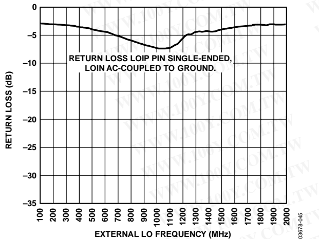
Figure 45. Return Loss of LOIP Input vs. External LO Frequency
