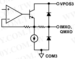
Figure 10. Circuit H
