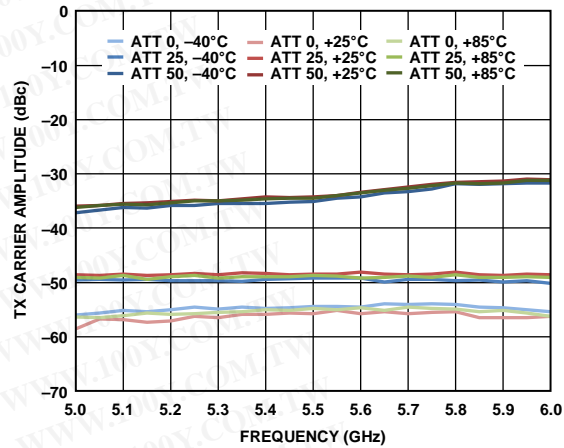
Figure 68. TX Carrier Rejection vs. Frequency
