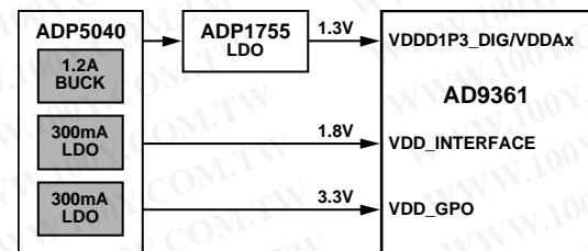
Figure 75. Space-Optimized Power Solution for the AD9361
