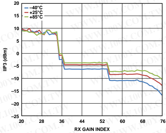
Figure 38. Third-Order Input Intercept Point (IIP3) vs. RX Gain Index, f_1 = 30 MHz, f_2 = 61 MHz
