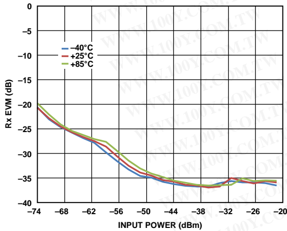
Figure 55. Rx EVM vs. Input Power, 64 QAM WiMAX 40 MHz Mode, 40 MHz REF_CLK (Doubled Internally for RF Synthesizer)
