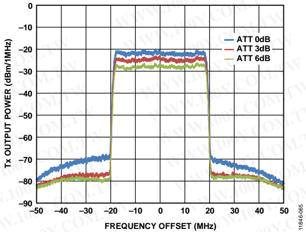
Figure 65. Tx Spectrum vs. Frequency Offset from Carrier Frequency, f_{LO\_TX} = 5.8 GHz, WiMAX 40 MHz Downlink (Digital Attenuation Variations Shown)
