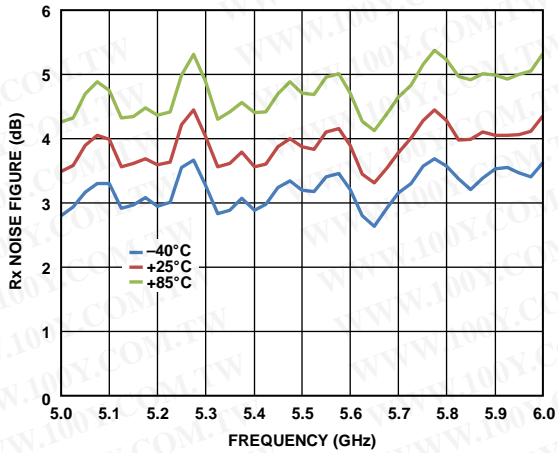
Figure 53. Rx Noise Figure vs. Frequency
