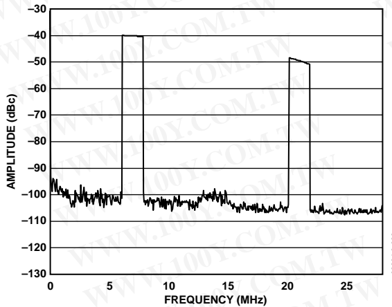
Figure 36. AD9863 Tx Path FFT of OFDM Signal in Figure 34, with 1x Interpolation
