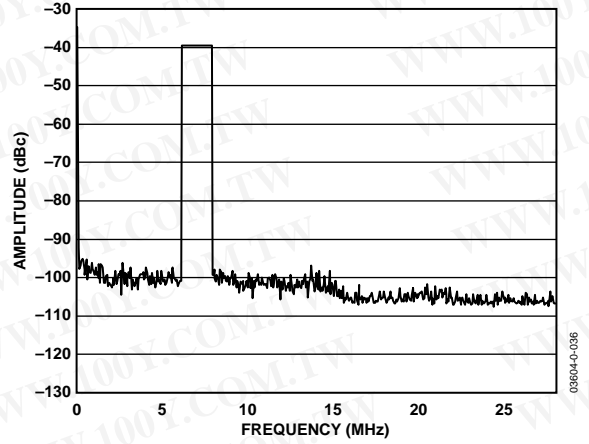
Figure 39. AD9863 Tx Path FFT of OFDM Signal in Figure 34, with 2x Interpolation
