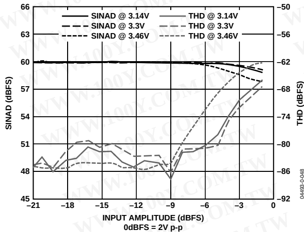
Figure 11. SINAD and THD vs. Input Amplitude and Supply ( f_{\text{IN}} = 8 MHz, \text{LPF } f_{-3\text{dB}} = 26 MHz; \text{RxPGA} = 0 dB)
