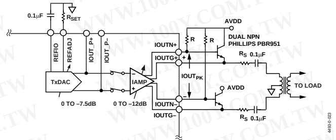
Figure 65. Voltage-Mode Operation
