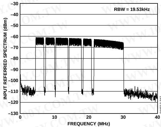
Figure 10. Spectral Plot with 4k FFT of 111-Carrier DMT Signal with \text{PAR} = 11 dB, P_{\text{IN}} = -33.7 dBm, \text{LPF } f_{-3\text{dB}} = 32 MHz, and \text{RxPGA} = 36 dB
