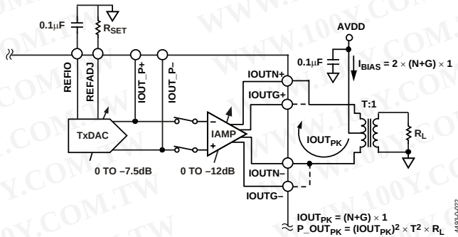
Figure 64. Current-Mode Operation
