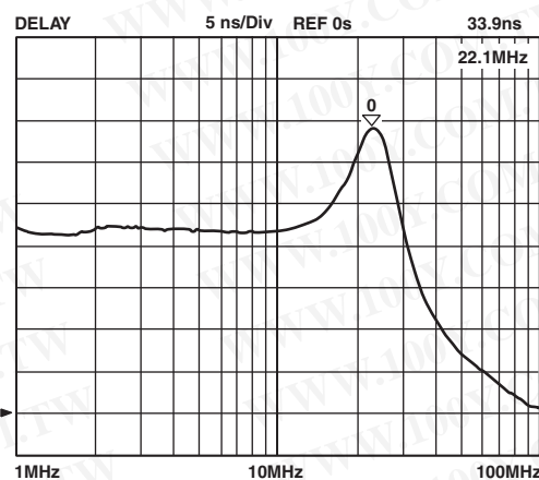
TPC 17. Rx LPF Group Delay, LPF = Wideband Rx Filter, F_{ADC} = 50 MHz, Tuning Target = 255
