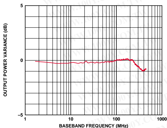
Figure 5. I and Q Input Bandwidth Normalized to Gain @ 1 MHz ( f_{\text{LO}} = 3500\text{ MHz} )
