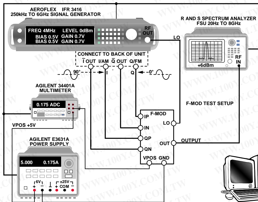
Figure 39. Characterization Bench Setup
