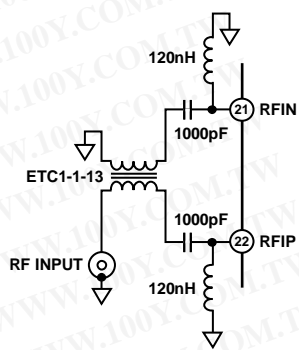
Figure 48. RF Input
