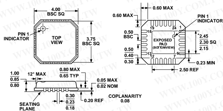
Figure 68. 24-Lead Lead Frame Chip Scale Package [LFCSP_VQ] 4 mm x 4 mm Body, Very Thin Quad (CP-24-2) Dimensions shown in millimeters
