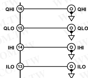
Figure 50. Baseband Output Configuration
