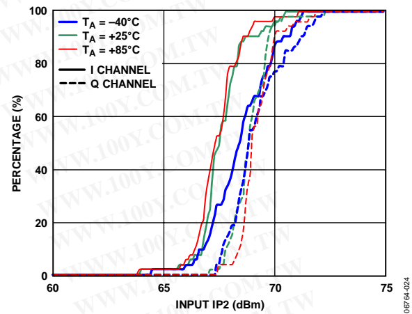
Figure 24. IIP2 Distributions for I Channel and Q Channel
