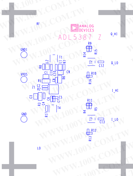
Figure 65. Evaluation Board Top Layer Silkscreen
