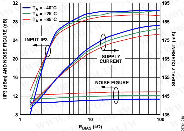
Figure 10. Noise Figure, IIP3, and Supply Current vs. R_{BIAS} , f_{RF} = 140 MHz
