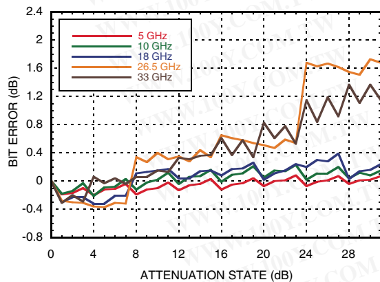
Bit Error vs. Attenuation State
