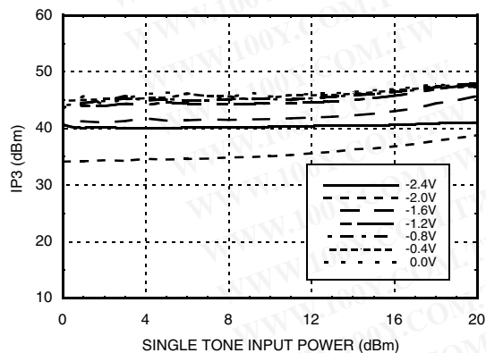
Input IP3 vs. Input Power @ 30 GHz Vctrl1 = Variable, Vctrl2 = -3V
