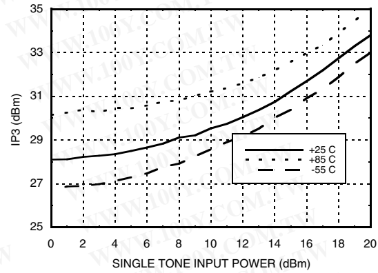
Input IP3 vs. Input Power Over Temperature @ 30 GHz Vctrl1 = Vctrl2
