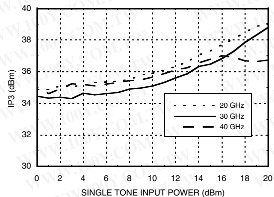
Input IP3 vs. Input Power @ 30 GHz Vctrl1 = -2V, Vctrl2 = -3V [1]
