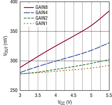
V_{OUT} Offset vs Supply Voltage
