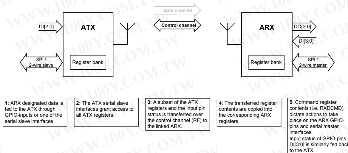
Figure 11. nRF24Z1 control channel transfer principle
