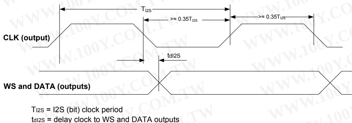
Figure 15. I2S output timing
