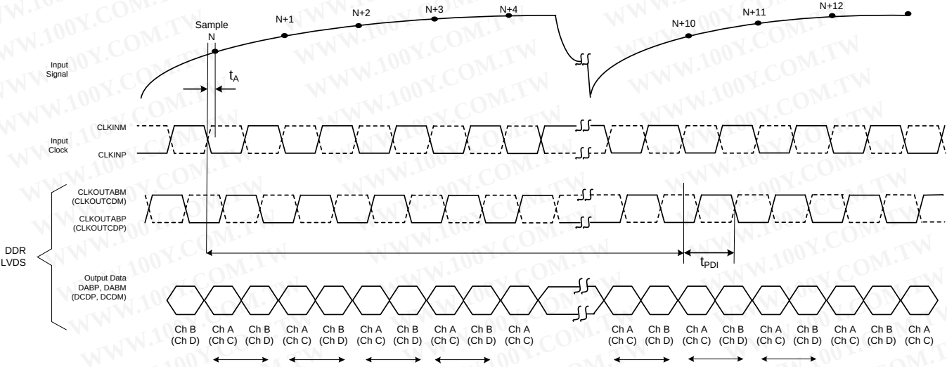
Figure 2. Latency Timing
