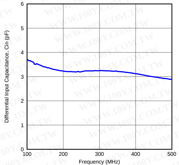
Figure 45. ADC Analog Input Capacitance ( C_{IN} ) vs Frequency
