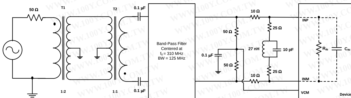
Figure 49. Driving Circuit for a 100- \Omega Source Impedance and Input Frequencies in the Third Nyquist Zone
