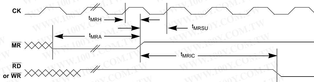
Figure 5. CLC5903 Master Reset Timing
