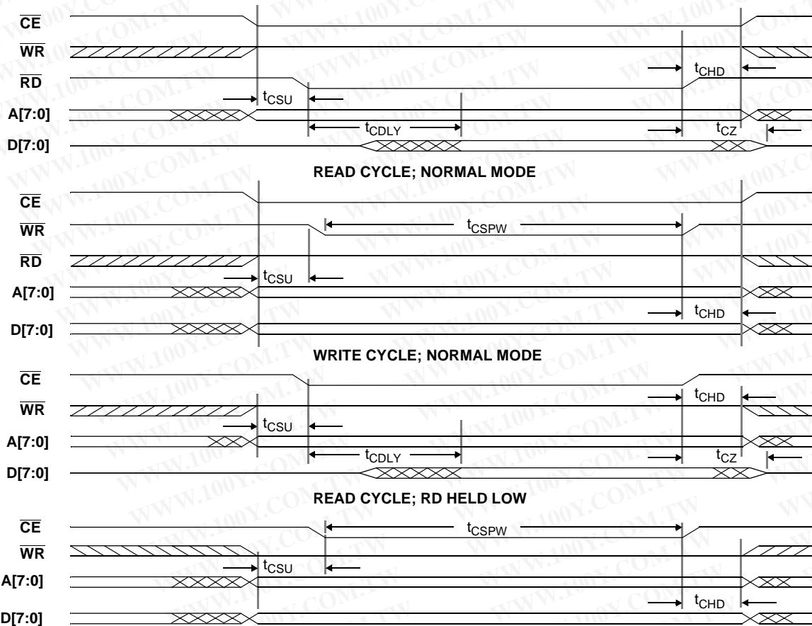
Figure 15. CLC5903 Control I/O Timing
