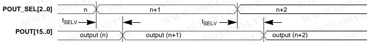
Figure 12. CLC5903 Parallel Output Select Timing
