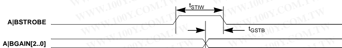
Figure 9. CLC5903 DVGA Interface Timing
