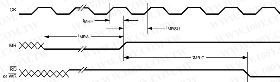
Figure 4. LM97593 Master Reset Timing
