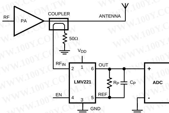
Figure 2. LMV221 with feedback (R)C Low Pass Filter
