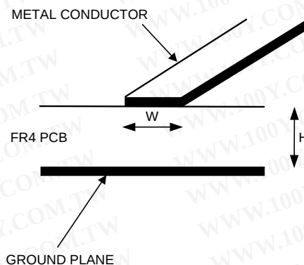
Figure 87. Microstrip Configuration
