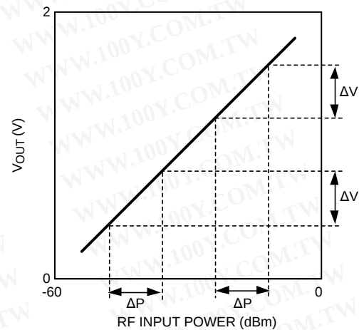
Figure 70. Linear Transfer Function
