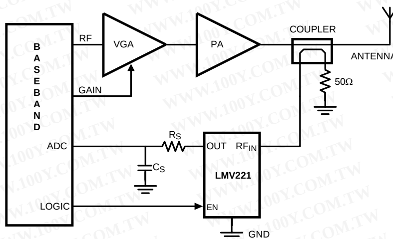
Figure 72. Transmit Power Control System
