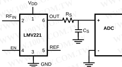
Figure 81. Low Pass Output Filter
