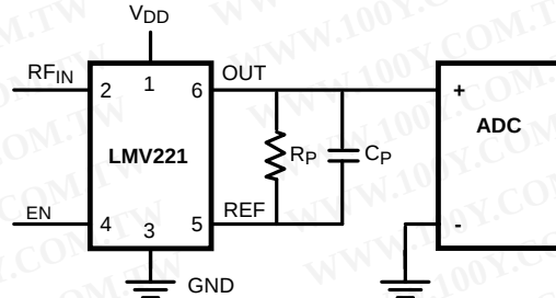
Figure 82. Low Pass Feedback Filter
