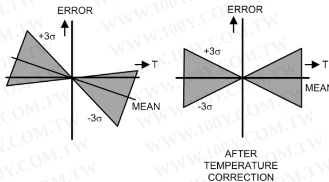
Figure 77. Elimination of the Systematic Component from the Temperature Drift
