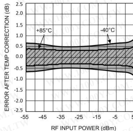
Figure 79. Temperature Drift Error with Temperature Compensation
