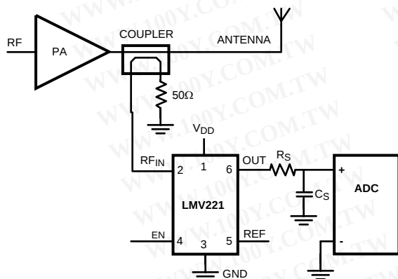
Figure 1. LMV221 with output RC Low Pass Filter
