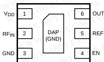
Figure 3. 6-pin WSON Top View
