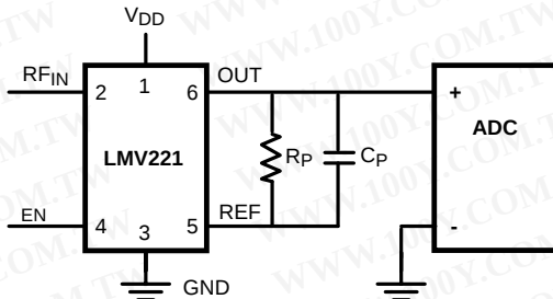
Figure 83. Single Ended Application
