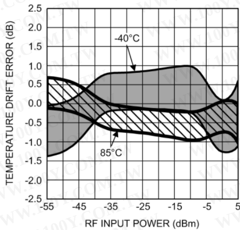
Figure 78. Temperature Drift Error without Temperature Compensation
