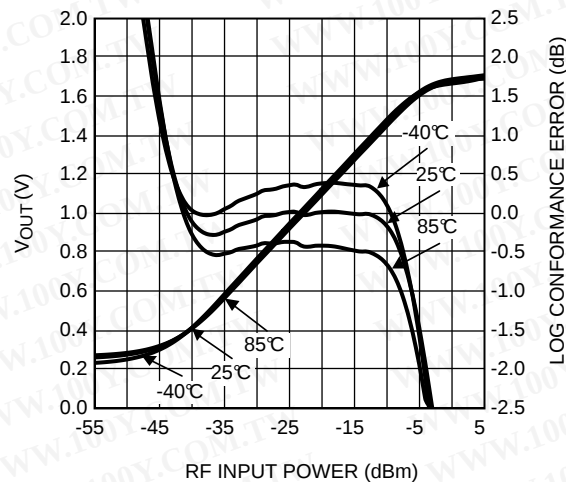
Figure 75. LOG-Conformance Error and LOG-Detector Transfer Function
