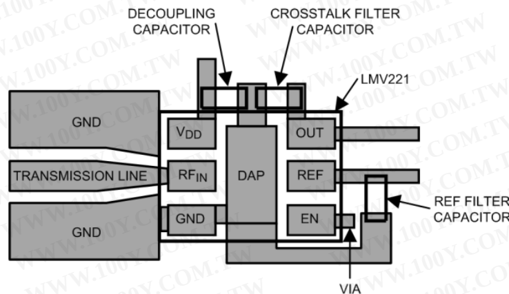
Figure 86. Recommended Board Layout
