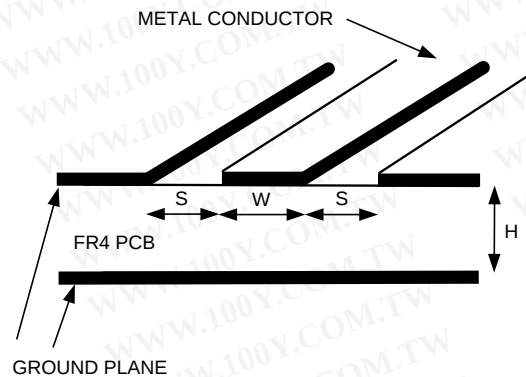
Figure 88. GCPW Configuration
