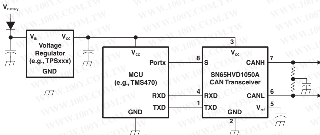
Figure 12. Typical Application
