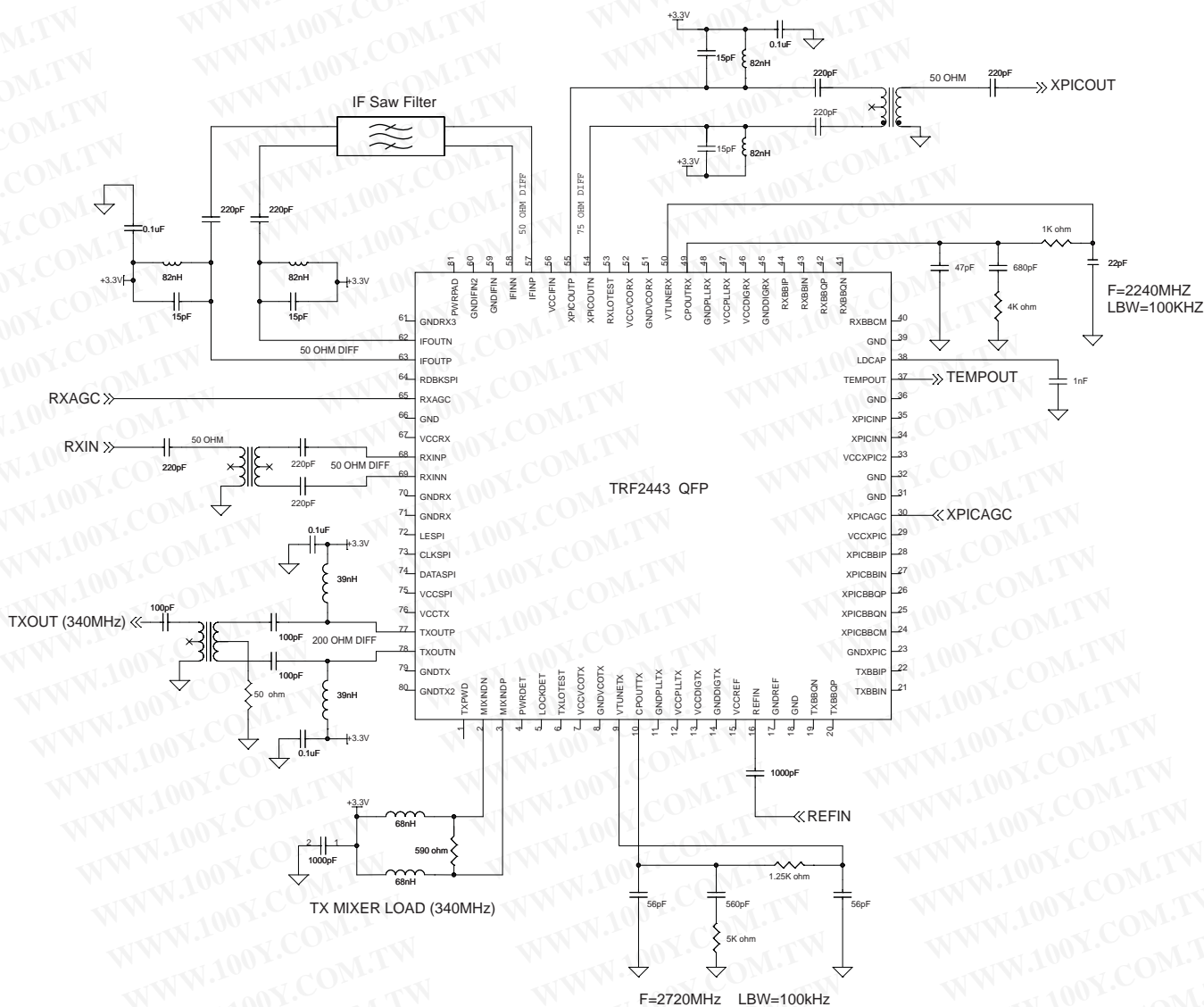
Figure 110. TRF2443 Application Schematic
