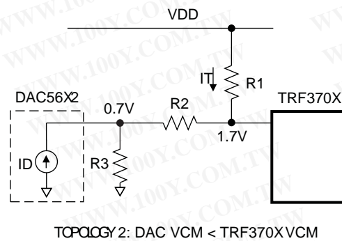
Figure 50. Passive DAC-to-Modulator Interface Network
