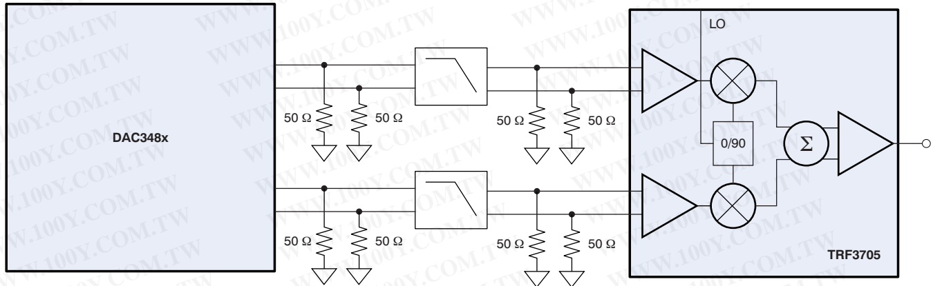
Figure 71. DAC348x Interface with the TRF3705 Modulator
