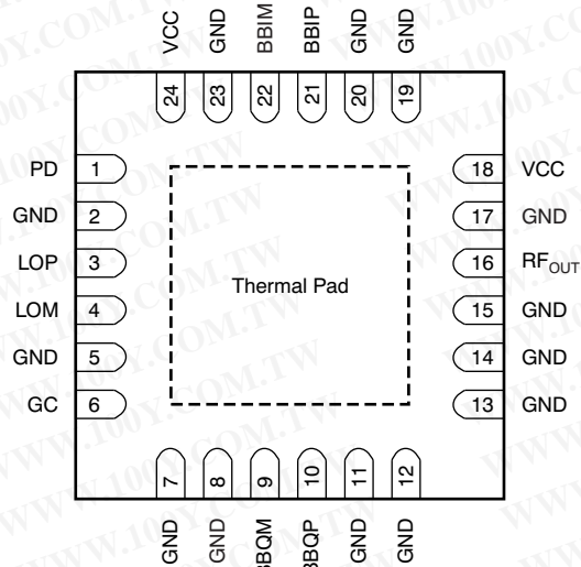
RGE PACKAGE VQFN-24 (TOP VIEW)
