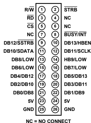
Figure 29. SKT4 Pinout
