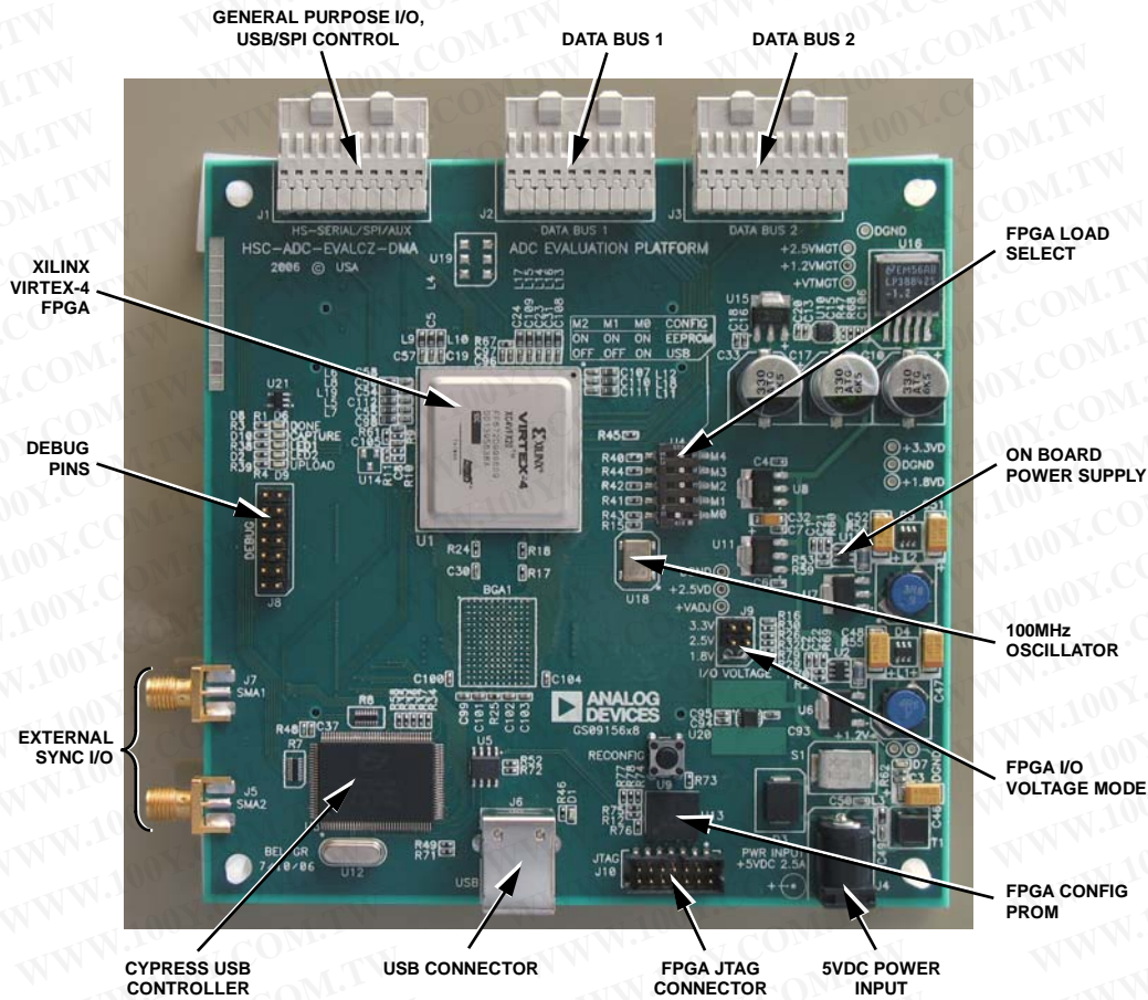
Figure 3. HSC-ADC-EVALC Components (Top View)
