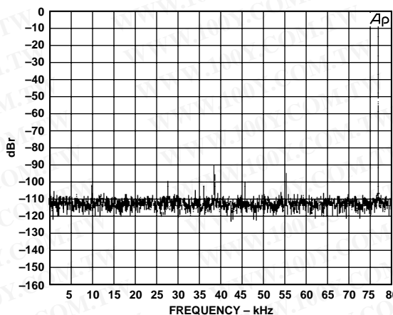
Figure 25. Wideband Plot, 75 kHz Input, 2x Interpolation, SR 192 kHz
