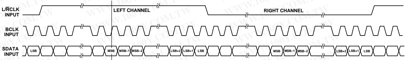
Figure 1. Right-Justified Mode
