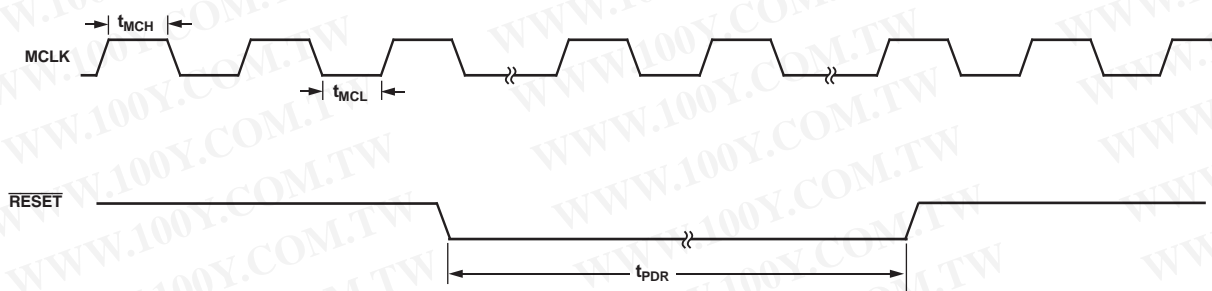
Figure 1. MCLK/RESET Timing
