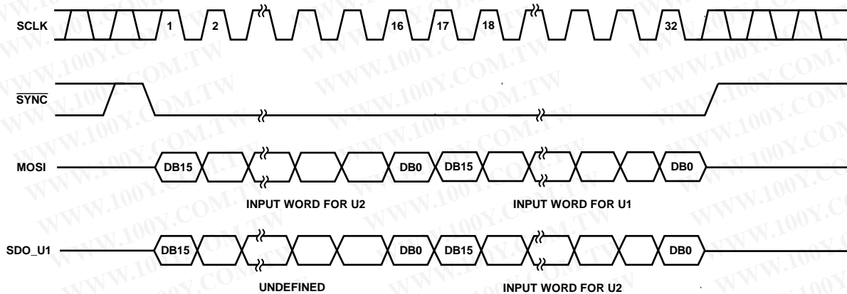
Figure 40. Daisy-Chain Diagram
