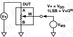
Figure 35. Potentiometer Divider Nonlinearity Error (INL, DNL)
