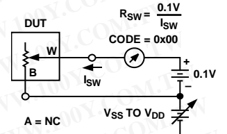
Figure 38. Incremental On Resistance
