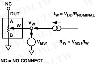
Figure 36. Wiper Resistance
