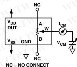
Figure 14. Common-Mode Leakage Current Test Circuit
