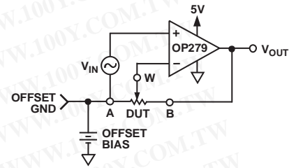
Figure 27. Noninverting Gain
