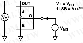
Figure 27. Potentiometer Divider Nonlinearity Error (INL, DNL)
