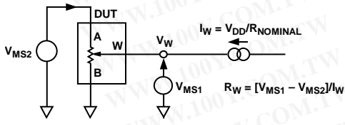
Figure 29. Wiper Resistance
