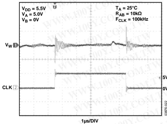
Figure 24. Digital Feedthrough
