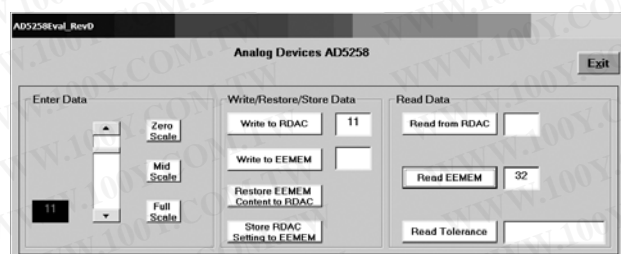
Figure 43. AD5258 Evaluation Board Software
