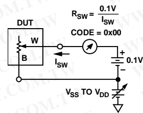
Figure 36. Test Circuit for Incremental On Resistance
