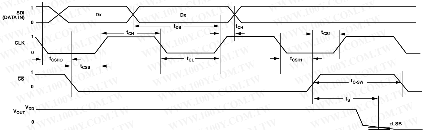
Figure 41. Detailed SPI Timing Diagram ( V_A = 5V, V_B = 0V, V_W = V_{OUT} )
