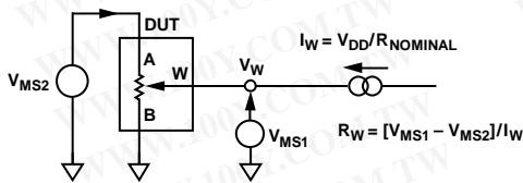
Figure 31. Test Circuit for Wiper Resistance
