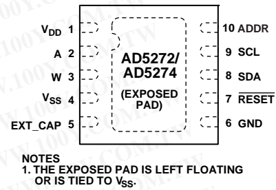
Figure 5. LFCSP Pin Configuration
