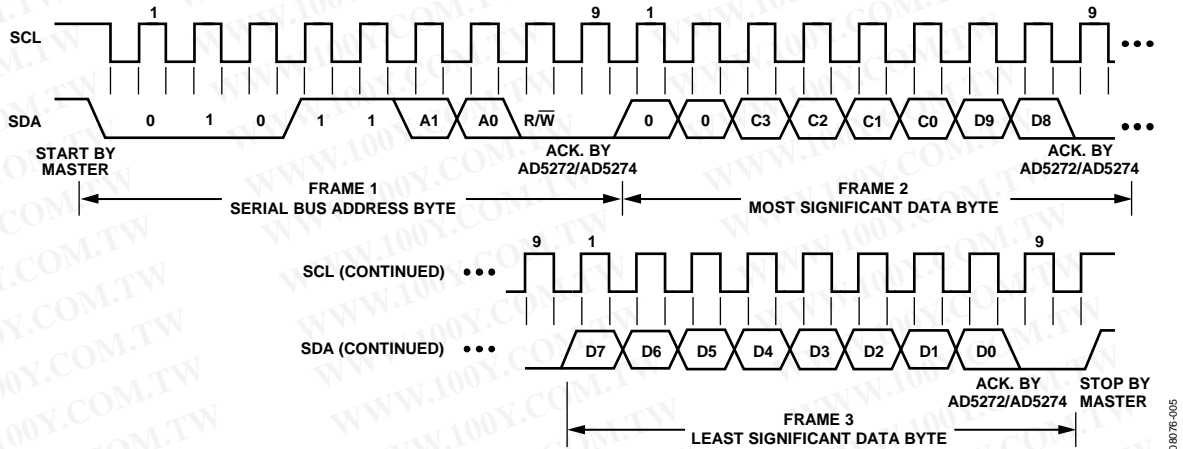
Figure 43. Write Command
