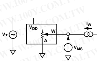
Figure 40. Power Supply Sensitivity (PSS, PSRR)
