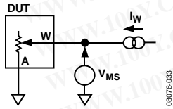
Figure 38. Resistor Position Nonlinearity (Rheostat Operation; R-INL, R-DNL)
