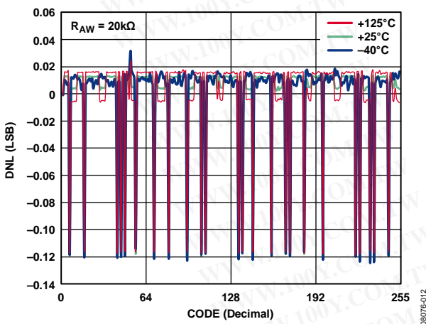
Figure 14. R-DNL in R-Perf Mode vs. Code vs. Temperature (AD5274)
