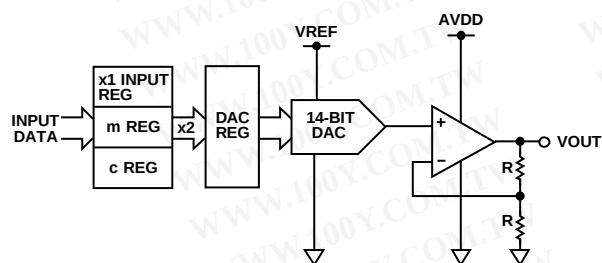
Figure 31. Single-Channel Architecture
