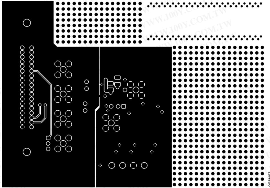
Figure 57. Solder-Side Artwork
