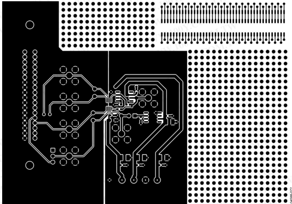
Figure 55. Component-Side Artwork
