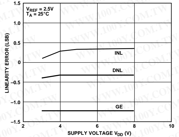
Figure 11. Linearity Error vs. V_{DD}
