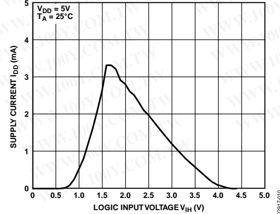
Figure 12. Supply Current vs. Logic Input Voltage
