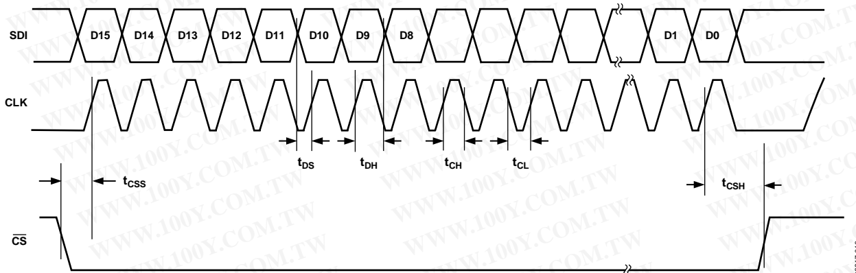
Figure 4. AD5543 Timing Diagram
