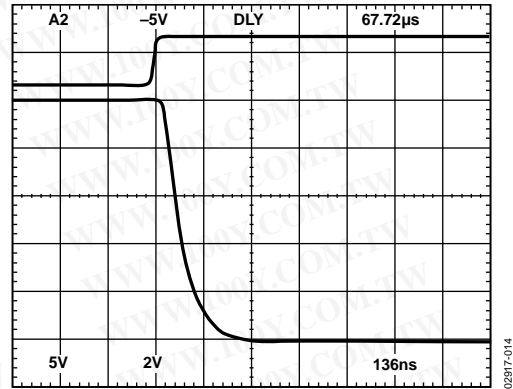
Figure 15. Settling Time
