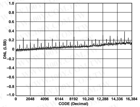
Figure 10. AD5553 Differential Nonlinearity Error
