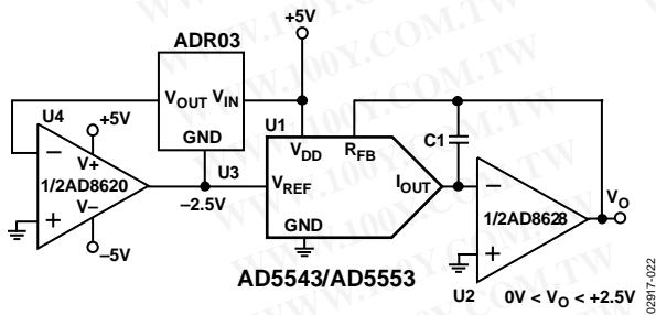
Figure 21. Positive Voltage Output Configuration
