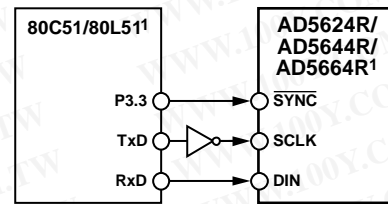
Figure 59. 80C51/80L51 Interface to AD5624R/AD5644R/AD5664R
