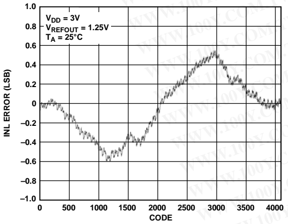
Figure 18. AD5624R-3 INL, Internal Reference
