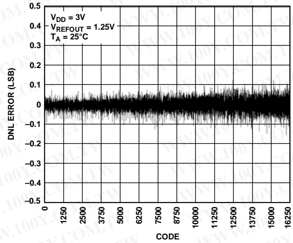
Figure 20. AD5644R-3 DNL, Internal Reference
