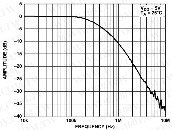
Figure 49. Multiplying Bandwidth
