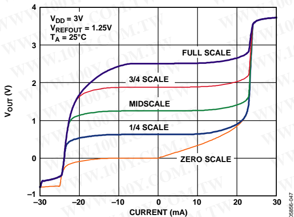
Figure 35. AD56x4R-3 Source and Sink Capability
