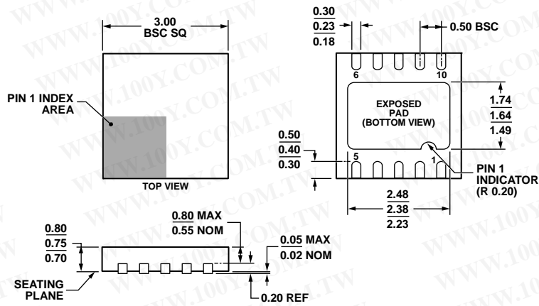
Figure 64. 10-Lead Lead Frame Chip Scale Package [LFCSP_WD] 3 mm x 3 mm Body, Very Very Thin, Dual Lead (CP-10-9) Dimensions shown in millimeters
