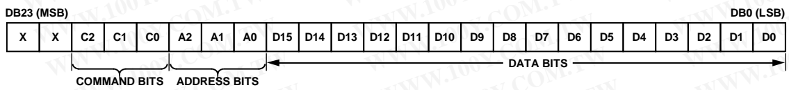
Figure 52. AD5664R Input Shift Register Contents
