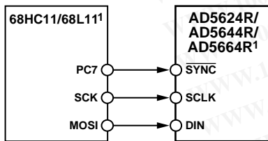
Figure 58. 68HC11/68L11 Interface to AD5624R/AD5644R/AD5664R
