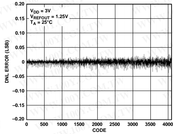
Figure 21. AD5624R-3 DNL, Internal Reference
