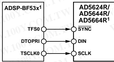
Figure 57. Blackfin ADSP-BF53x Interface to AD5624R/AD5644R/AD5664R
