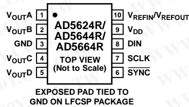
Figure 3. Pin Configuration
