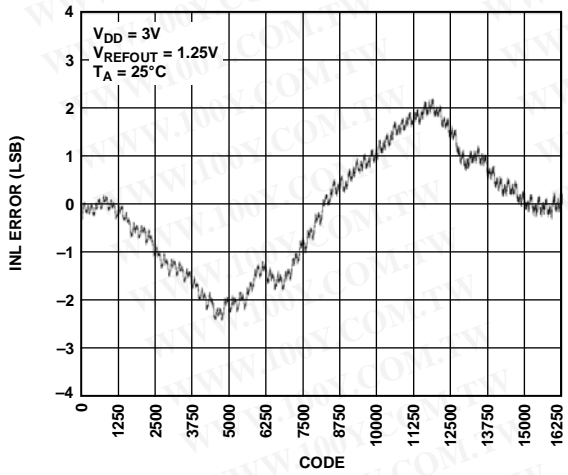
Figure 17. AD5644R-3 INL, Internal Reference
