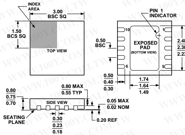
Figure 42. 10-Lead Lead Frame Chip Scale Package [LFCSP_WD] 3 mm × 3 mm Body, Very Very Thin, Dual Lead (CP-10-9) Dimensions shown in millimeters
