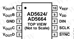
Figure 3. Pin Configuration
