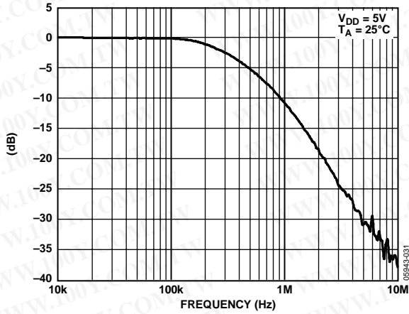
Figure 28. Multiplying Bandwidth
