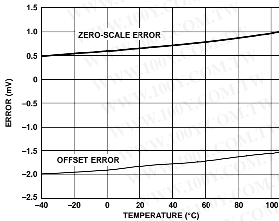
Figure 12. Zero-Scale Error and Offset Error vs. Temperature
