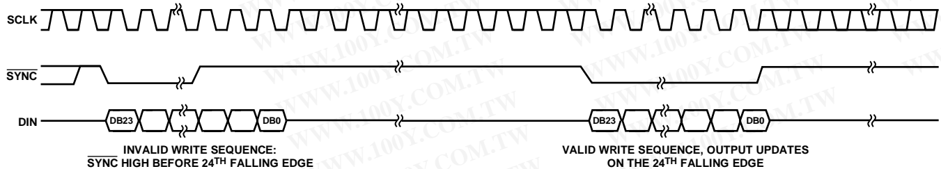
Figure 33. SYNC Interrupt Facility
