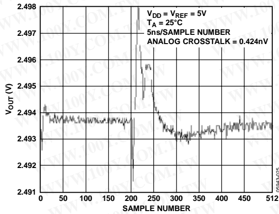
Figure 23. Analog Crosstalk
