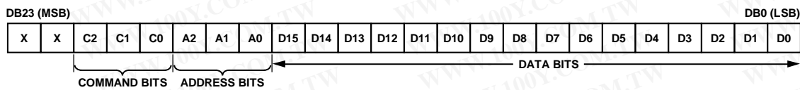
Figure 31. AD5664 Input Shift Register Contents
