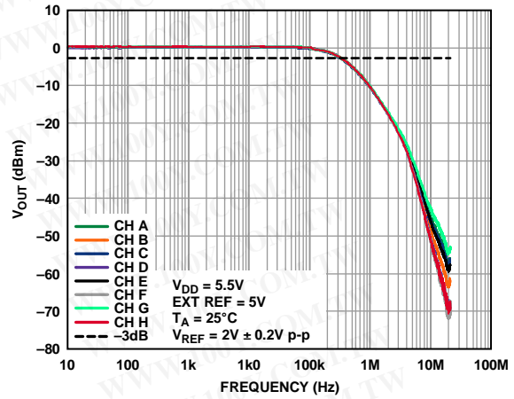
Figure 51. Multiplying Bandwidth
