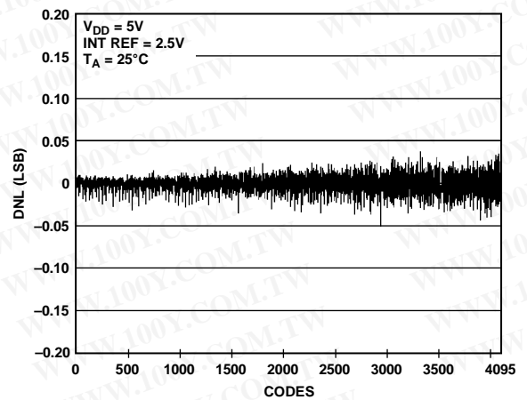
Figure 17. DNL AD5628-2
