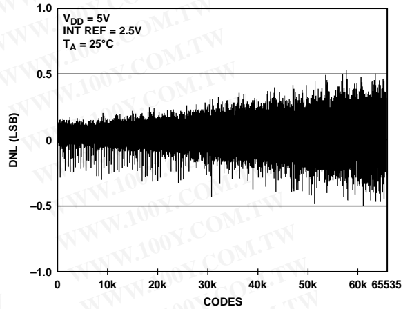
Figure 15. DNL AD5668-2/AD5668-3
