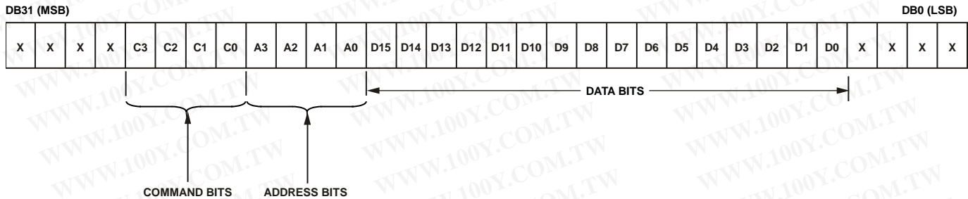
Figure 56. AD5668 Input Register Contents
