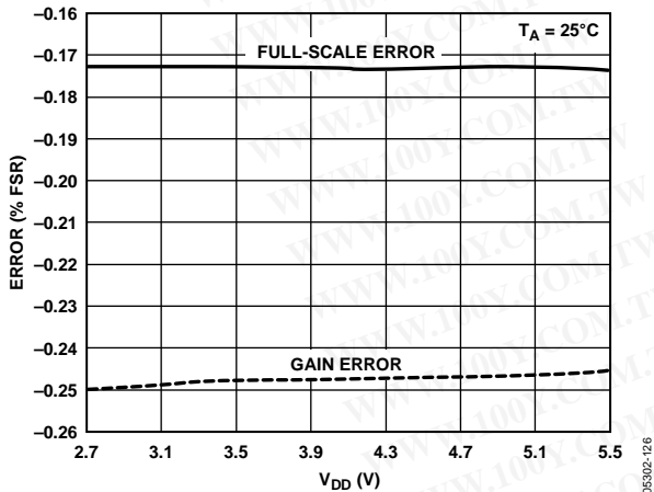
Figure 26. Gain Error and Full-Scale Error vs. Supply Voltage
