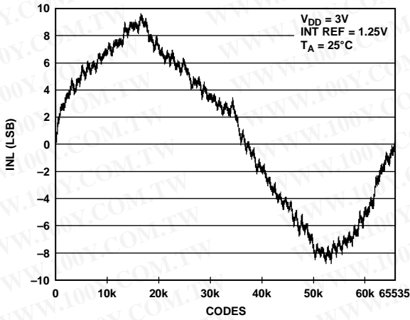
Figure 18. INL AD5668-1
