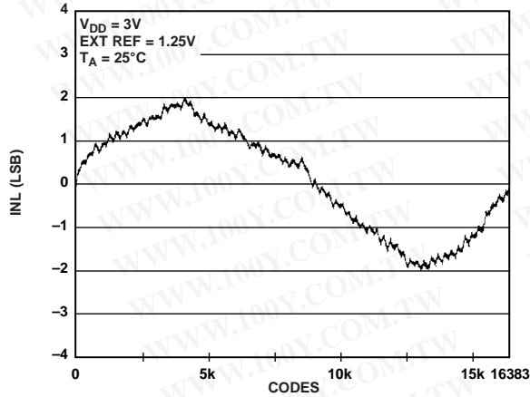
Figure 19. INL AD5648-1
