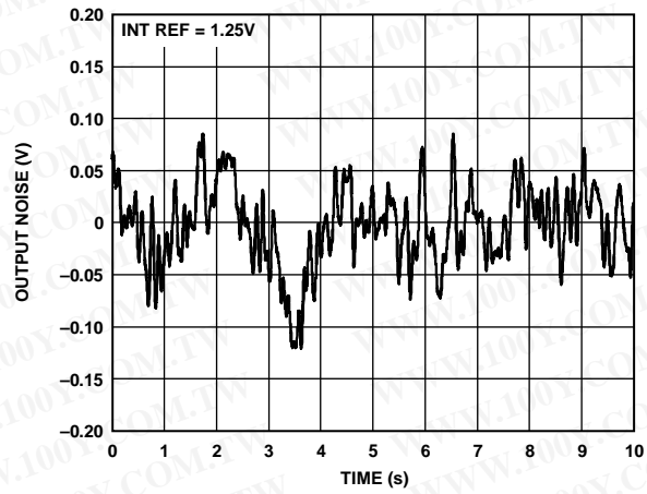
Figure 46. 0.1 Hz to 10 Hz Output Noise Plot, Internal Reference
