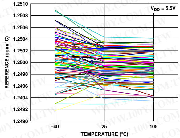
Figure 52. 1.25 V Reference Temperature Coefficient vs. Temperature
