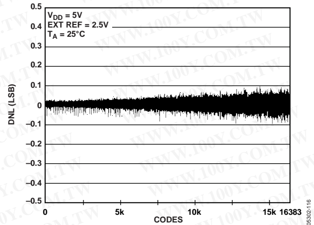
Figure 16. DNL AD5648-2
