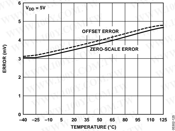
Figure 25. Zero-Scale Error and Offset Error vs. Temperature
