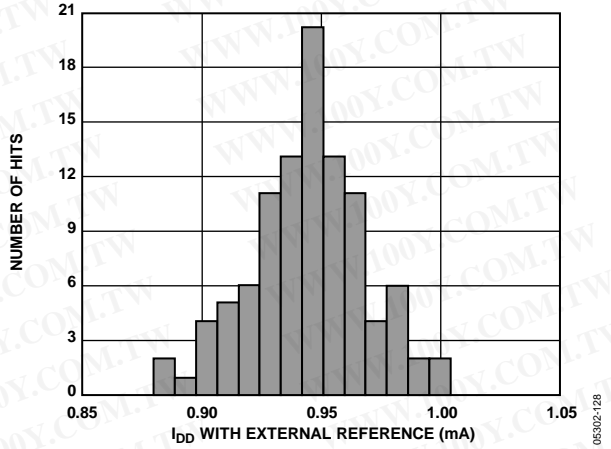
Figure 28. I_{DD} Histogram with External Reference
