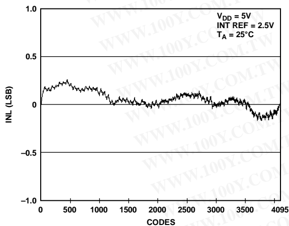
Figure 14. INL AD5628-2
