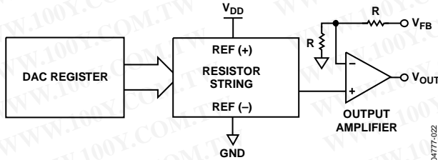
Figure 32. DAC Architecture
